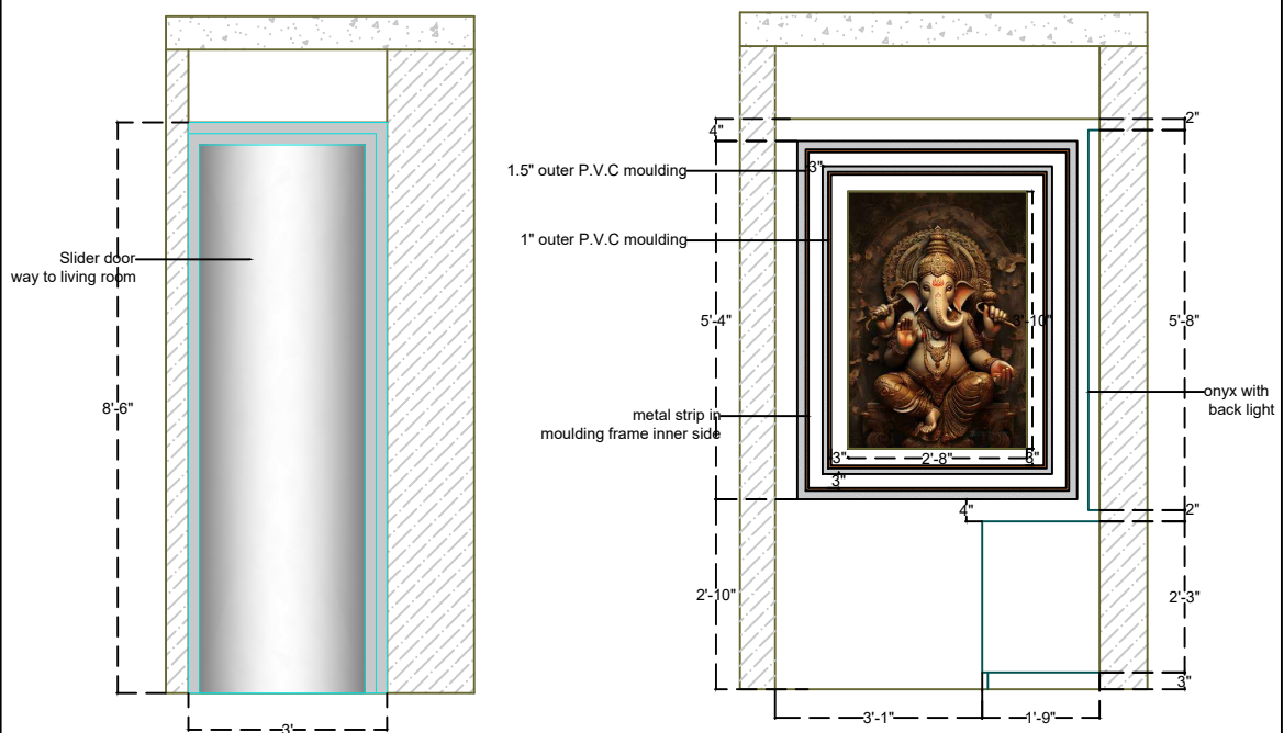
Elevation C
