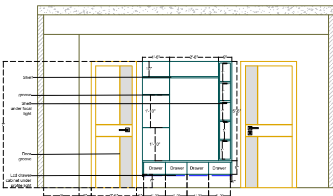
Elevation C
