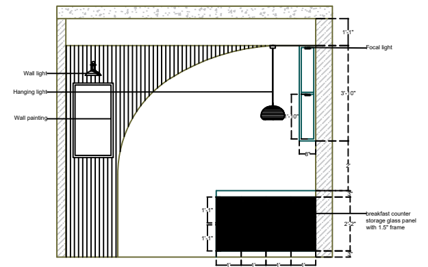
Elevation D
