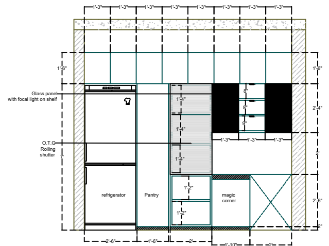
Elevation D
