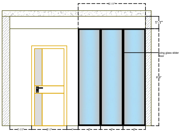
Elevation C
