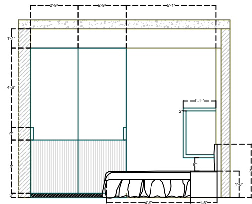
Elevation D
